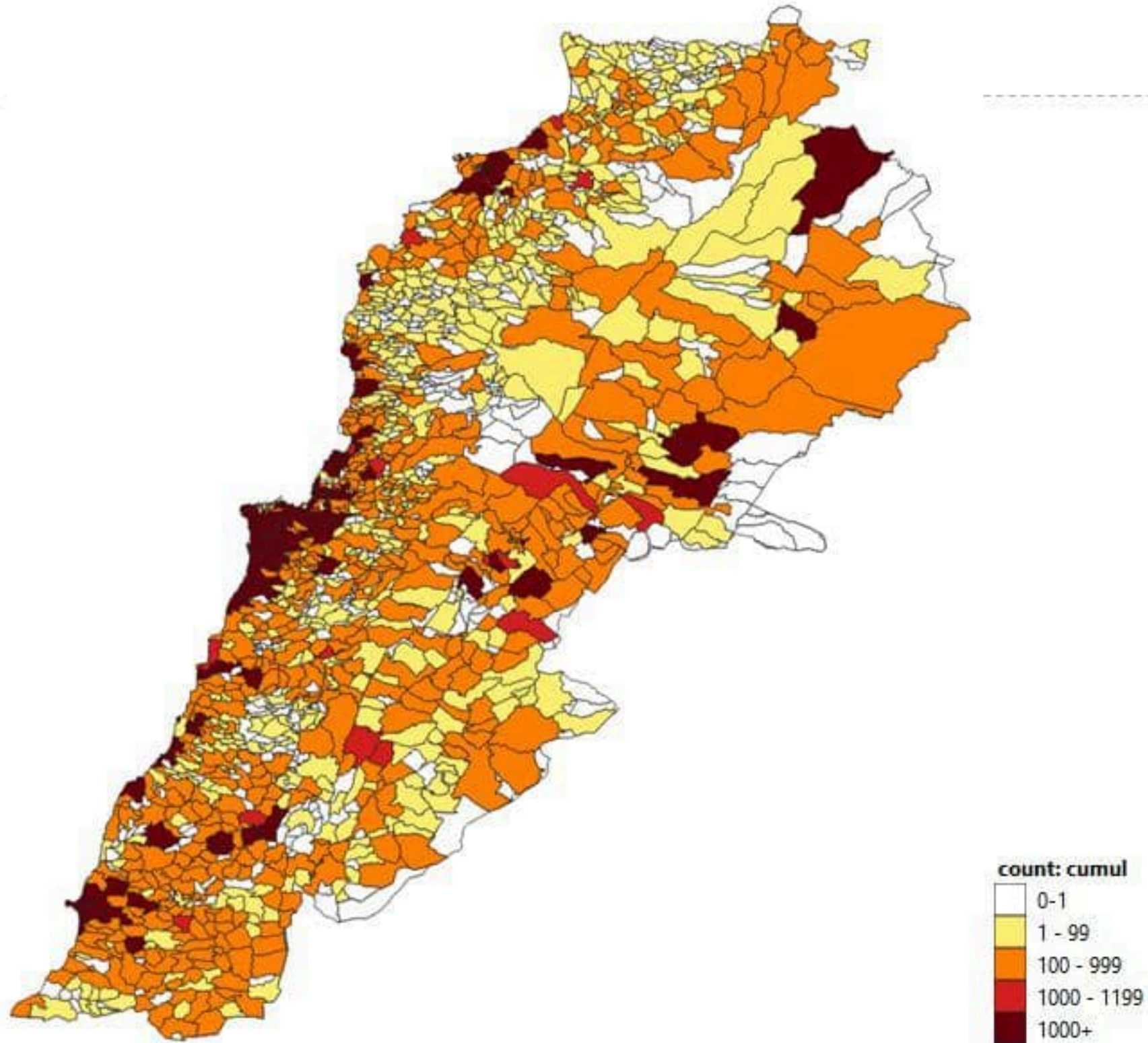
Map of distribution of cumulative number of cases by locality – 07 December 2021
